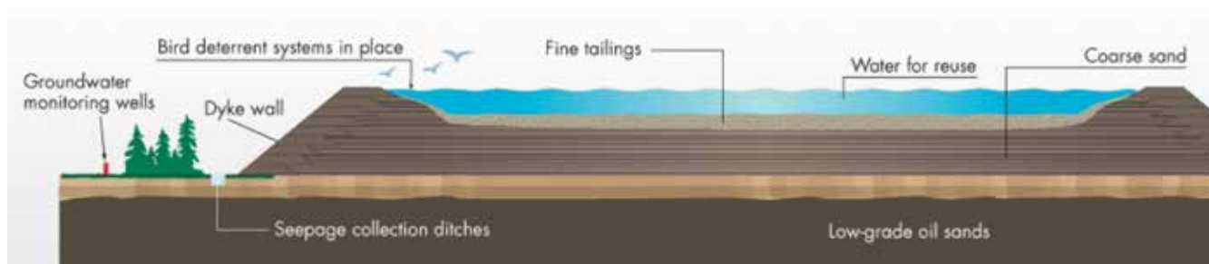
Figure 4.8: Tailings Pond. Source: Oil Sands Today
